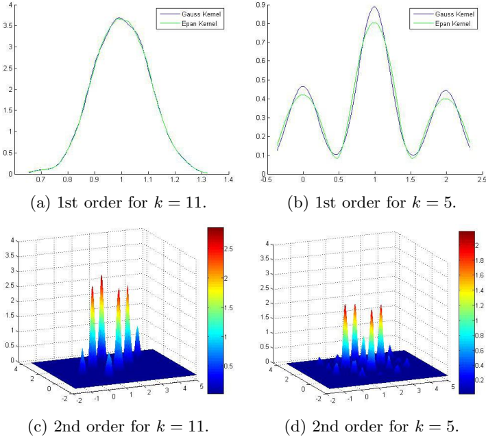
Fig. 3. Kernel Method
