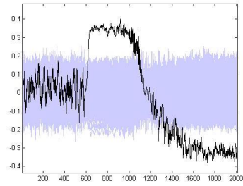
(b) CPA(HW) attack with 256 traces.
