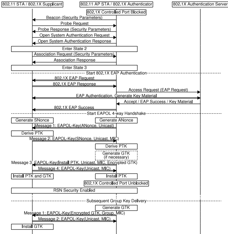
Fig. 3. 802.11i RSN authentication and key management. Single lines represent management frames, double lines represent data frames. Note that a deauthentication attack will force the station to do the whole procedure over again, starting with the authentication request. If pairwise master key security association (PMKSA) caching is enabled, the 802.1X authentication does not have to be repeated.
