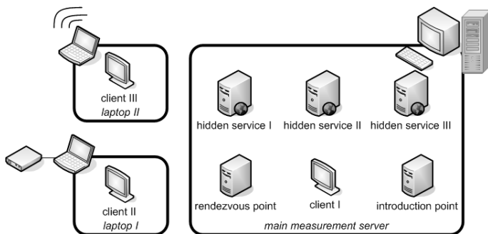
Fig. 3. Process distribution with clients using low-bandwidth access networks
