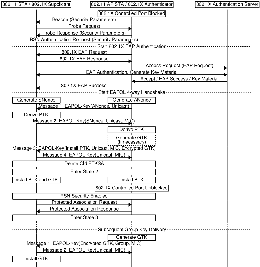
Fig. 9. The proposed solution for RSN authentication and key management. The authentication procedure is initiated when the station transmits an authentication frame with authentication algorithm number equal to 2 and a valid RSN information element. Management frames of subtype “authentication and key management” are used to encapsulate the 802.1X authentication messages, the 4-way handshake and the group key handshake. Note that the association request and response are protected.
